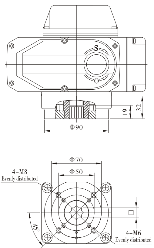
Direct installation type
